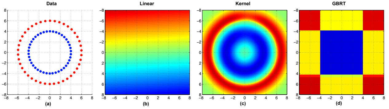
Figure 2.1: Gradient surface of a linear, a kernel and a GBRT classifier. (a) The linear un-separable simulation data. Red dots and blue dots are from two different classes, and the task is binary classification. (b) The gradient surface of a linear classifier, which is a hyper-plane (c) The gradient surface of a kernel classifier. (d) The gradient surface of a GBRT classifier.
