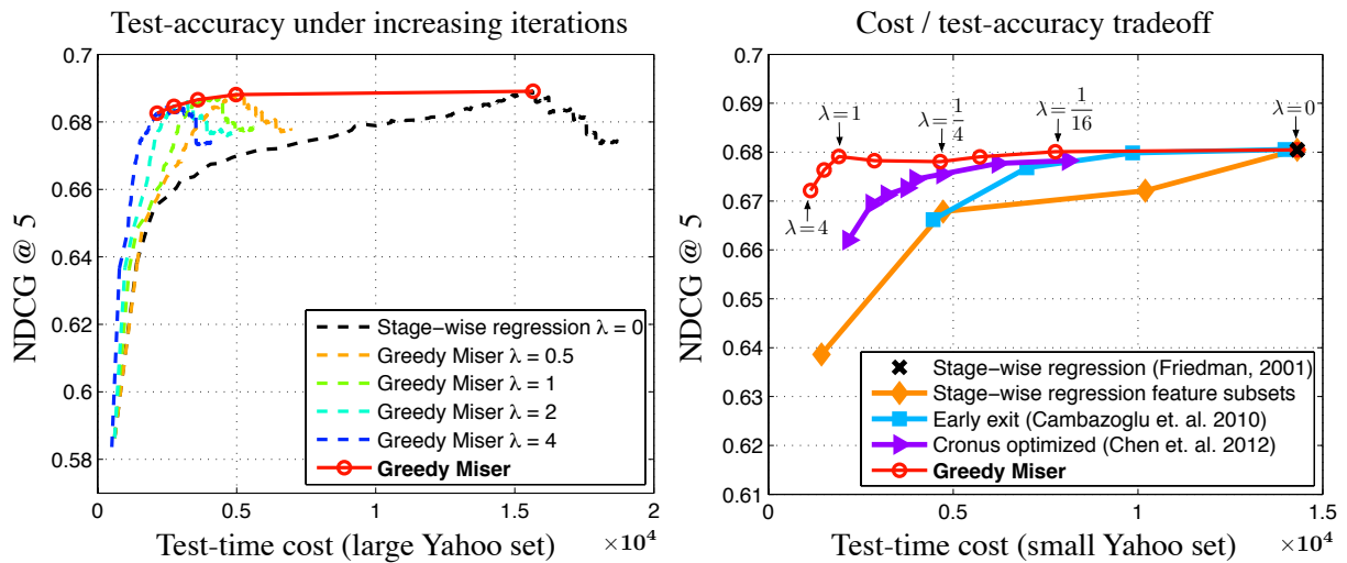
Figure 2.2: The NDCG@5 and the test-time cost of various classifier settings. Left: The comparison of the original Stage-wise regression ( \lambda = 0 ) and Greedy Miser under various feature-cost/accuracy trade-off settings ( \lambda ) on the full Yahoo set. The dashed lines represent the NDCG@5 as trees are added to the classifier. The red circles indicate the best scoring iteration on the validation data set. Right: Comparisons with prior work on test-time optimized cascades on the small Yahoo set. The cost-efficiency curve of Greedy Miser is consistently above prior work, reducing the cost, at similar ranking accuracy, by a factor of 10.
