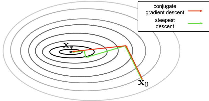
Figure 1.5: A schematic comparison of conjugate gradient descent (red) and steepest descent with line search (green).
